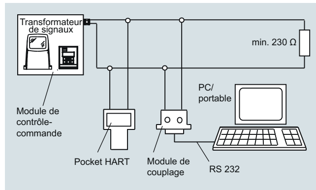
Communication HART
