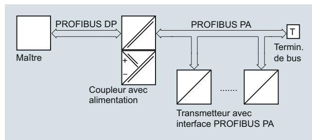
Communication PROFIBUS PA
